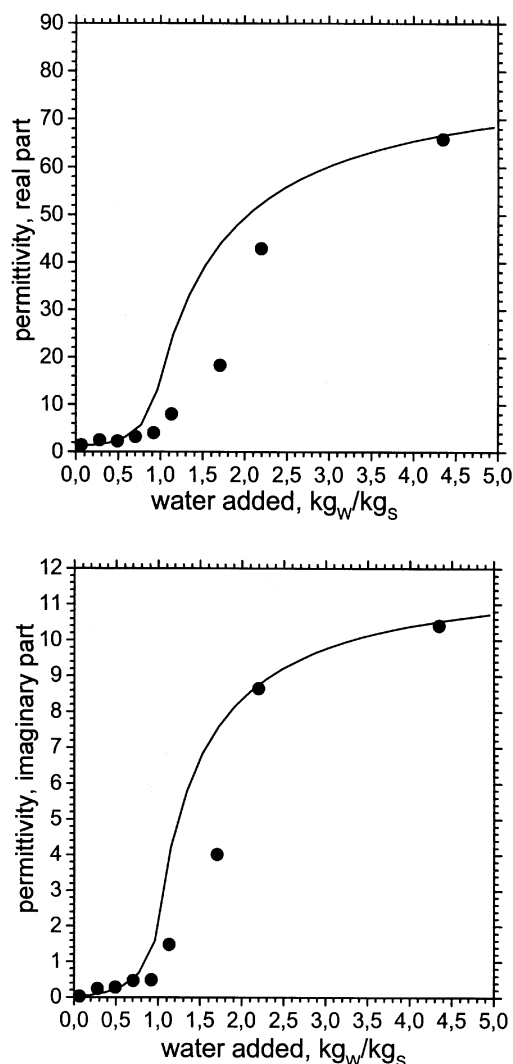
Figure 11. Real and imaginary part of the complex permittivity as a function of the water content (model curve: -; experimental ●) @ 2.45 GHz and 25°C.
