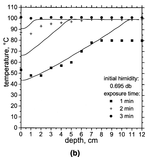
Figure 9. Model predictions of temperature profiles as a function of the depth for different initial moisture content and exposure time.
