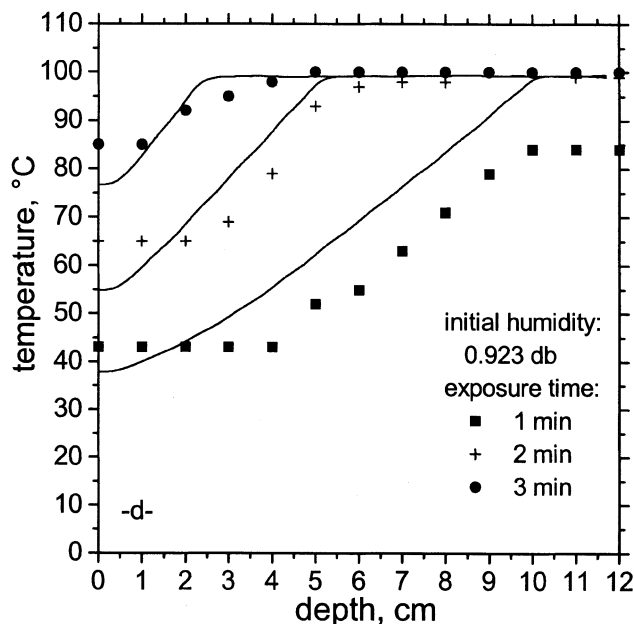
Figure 12. Model predictions of temperature profiles as a function of the depth for different initial moisture content and exposure time. Humidity is indicated on dry basis (db).
